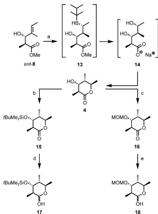
Scheme 3. a) (Thexyl)BH 2 (2.0 equiv), addition of ent - 8 , 0 °C, 30 min, → RT, 16 h; → 0 °C, NaOH (9M, 8.4 equiv), 35 % H 2 O 2 (9.2 equiv), NaCl (1.0 equiv), 2 h, → RT, 2 h; conc. HCl until pH ≤ 1; 60% ( ds > 98:2). b) t BuMe 2 SiOTf (2.6 equiv), 2,6-lutidine (1.5 equiv), CH 2 Cl 2 , 0 °C, 12 h; 72%. c) MOMCl (8.2 equiv), NEt 3 Pr 2 (8.7 equiv), n Bu 4 NI (1.1 mol %), CH 2 Cl 2 , RT, 1.5 h; 99%. d) DIBAL (2.2 equiv), toluene, –78 °C, 2.5 h; 99%. e) Same as d); 99%.
