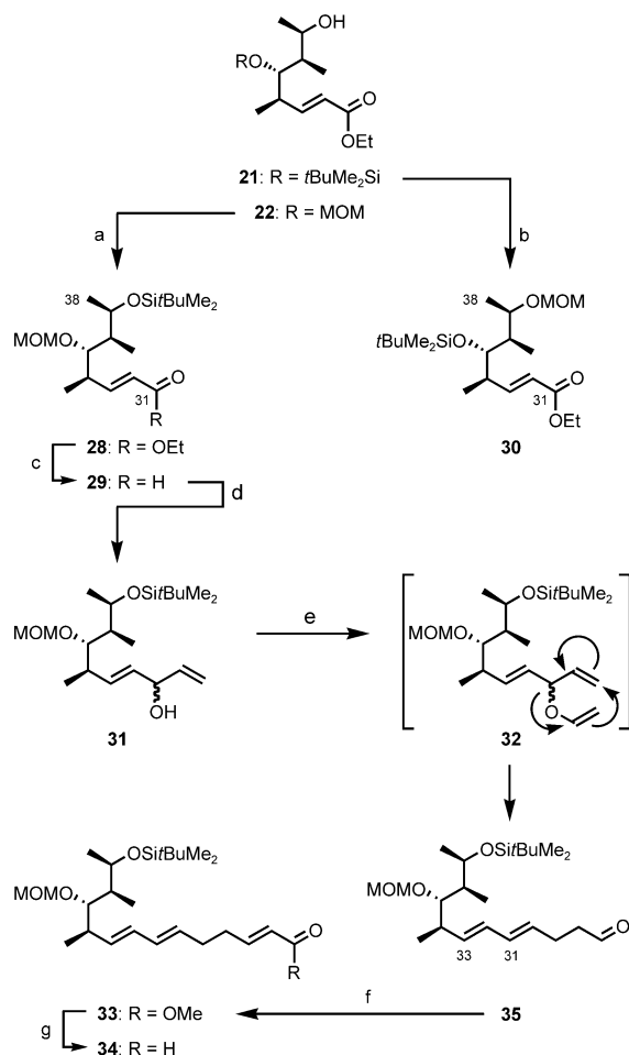
Scheme 4. a) t BuMe 2 SiOTf (2.0 equiv), 2,6-lutidine (3.6 equiv), CH 2 Cl 2 , 0 °C, 15 h; 84 %. b) MOMCl (8.3 equiv), NEt 3 Pr 2 (10 equiv), n Bu 4 NI (14 mol %), CH 2 Cl 2 , RT, 18 h; 85 %. c) (i) DIBAL (3.1 equiv), CH 2 Cl 2 , 78 °C, 1.5 h; (ii) MnO 2 (22 equiv), CH 2 Cl 2 , RT, 4 h; 89 %. d) H 2 C=CH-MgBr (2.3 equiv), THF, -78 °C, 70 min; 93 % ( ds ≈ 50:50). e) Hg(OAc) 2 (1.1 equiv), tert -butyl vinyl ether (70 equiv), reflux, 9 h; 78 %. f) Ph 3 P=CH-CO 2 Me (3.1 equiv), toluene, RT, 16 h; 89 % ( trans:cis > 98:2). g) i) DIBAL (2.6 equiv), CH 2 Cl 2 , -78 °C, 2.5 h; ii) MnO 2 (20 equiv), CH 2 Cl 2 , RT, 14 h; 89 %.
