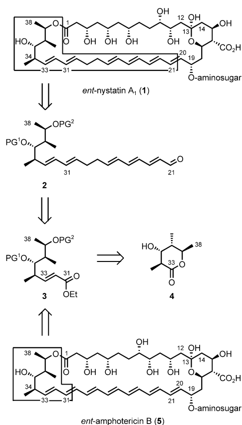
Scheme 1. Unnatural enantiomers 1 of nystatin A 1 and 5 of amphotericin B and retrosynthetic analysis of the boxed sections of these species.
