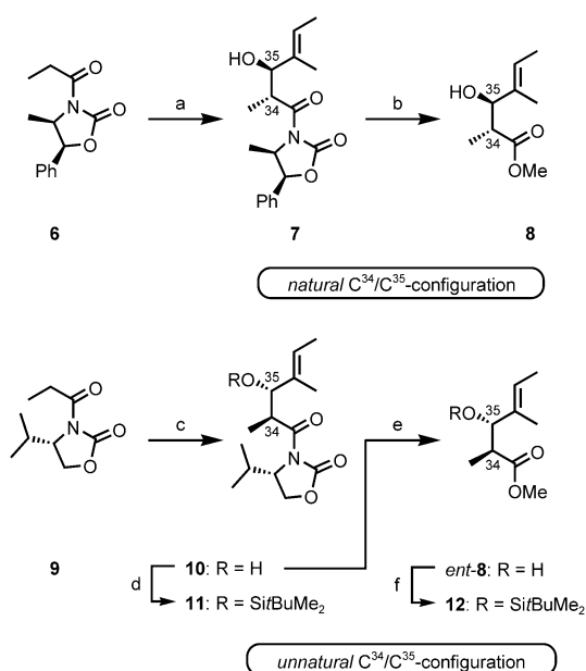
Scheme 2. a) NEt 3 (1.2 equiv), n Bu 2 BOTf (1.1 equiv), CH 2 Cl 2 , 0°C, 1 h, → -78°C; ( E )-2-methyl-2-butenal (1.15 equiv), → 0°C within 1 h; 0°C, 1 h; phosphate buffer (pH 7), MeOH, 35% H 2 O 2 , 1 h; 88% ( ds > 98:2). b) NaOMe (1.6 equiv), MeOH, 0°C, 8 min; 75%. c) Same as a); 96% ( ds > 98:2). d) t BuMe 2 SiOTf (1.5 equiv), 2,6-lutidine (2.2 equiv), CH 2 Cl 2 , 0°C, 1.5 h; 94%. e) Same as b); 86%. f) Same as d); 99%.
